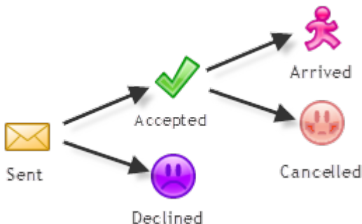
RSVP workflow
